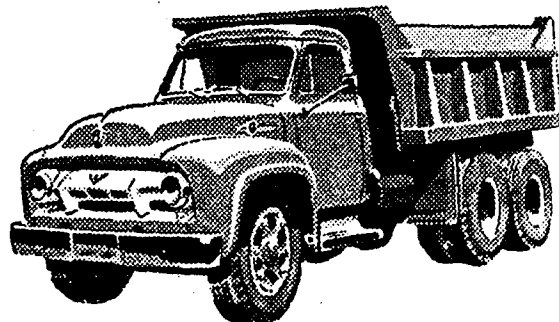
New Power Steering standard at no extra cost on new tandem-axle Ford T-800, GVW 40,000 lbs. Overhead-valve 170-h.p. V-8.
