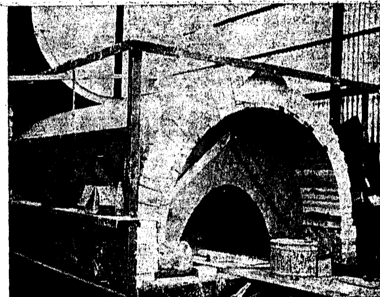
Brick furnace surrounding the boiler, in early stages of construction. The fire brick for this unit was produced at Troy, Idaho
